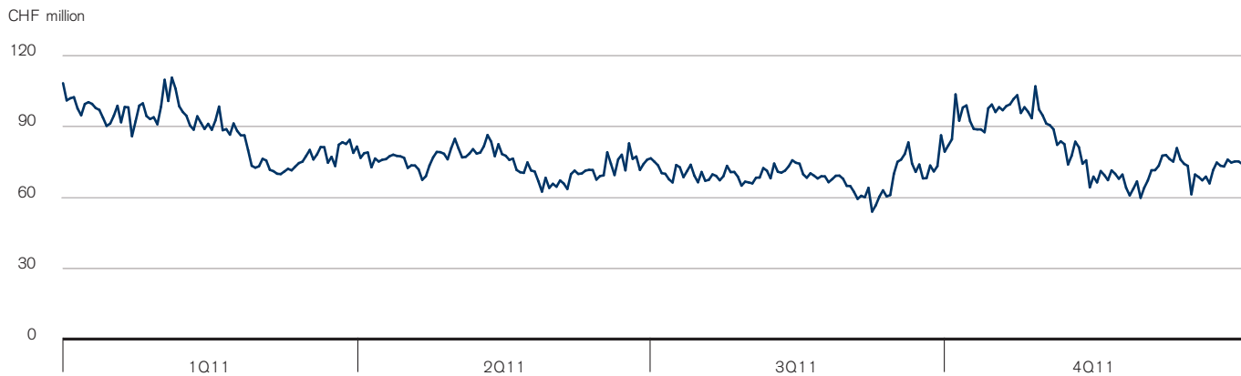
— One-day risk management VaR (98%)
